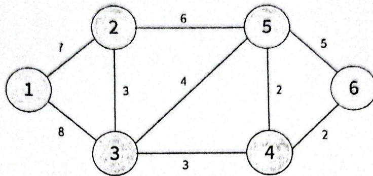
Graph G
